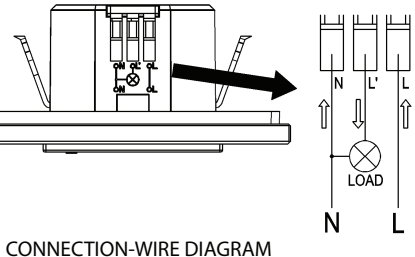
CONNECTION-WIRE DIAGRAM
